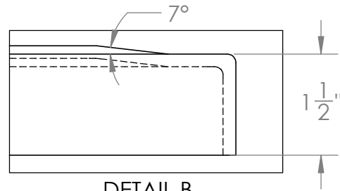
DETAIL B
