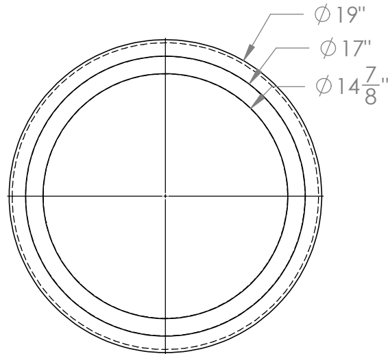
DETAIL B
