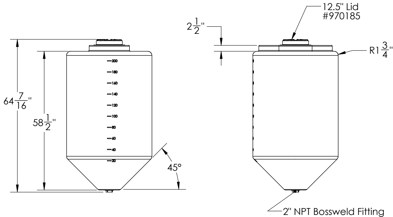
200 Gal. Cone Bottom Tank with 12.5" Lid & 2" FPT Bossweld Fitting
