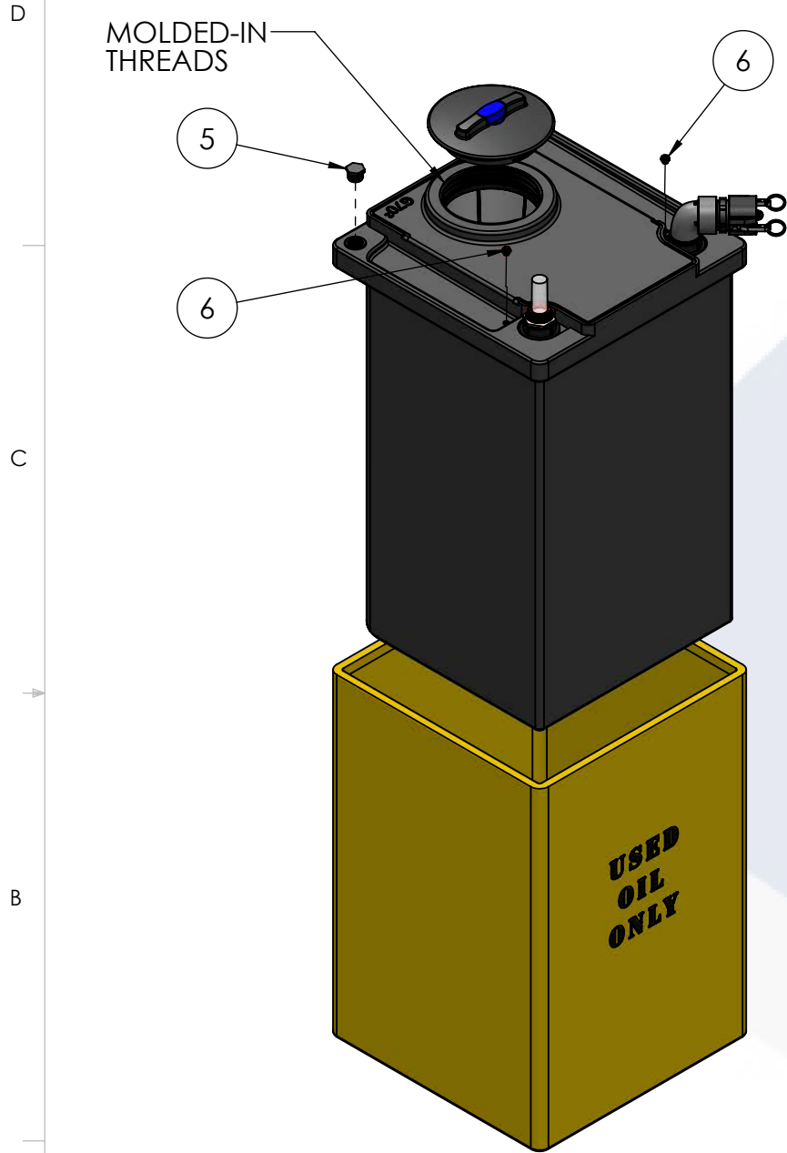
ISOMETRIC VIEW ASSEMBLED
