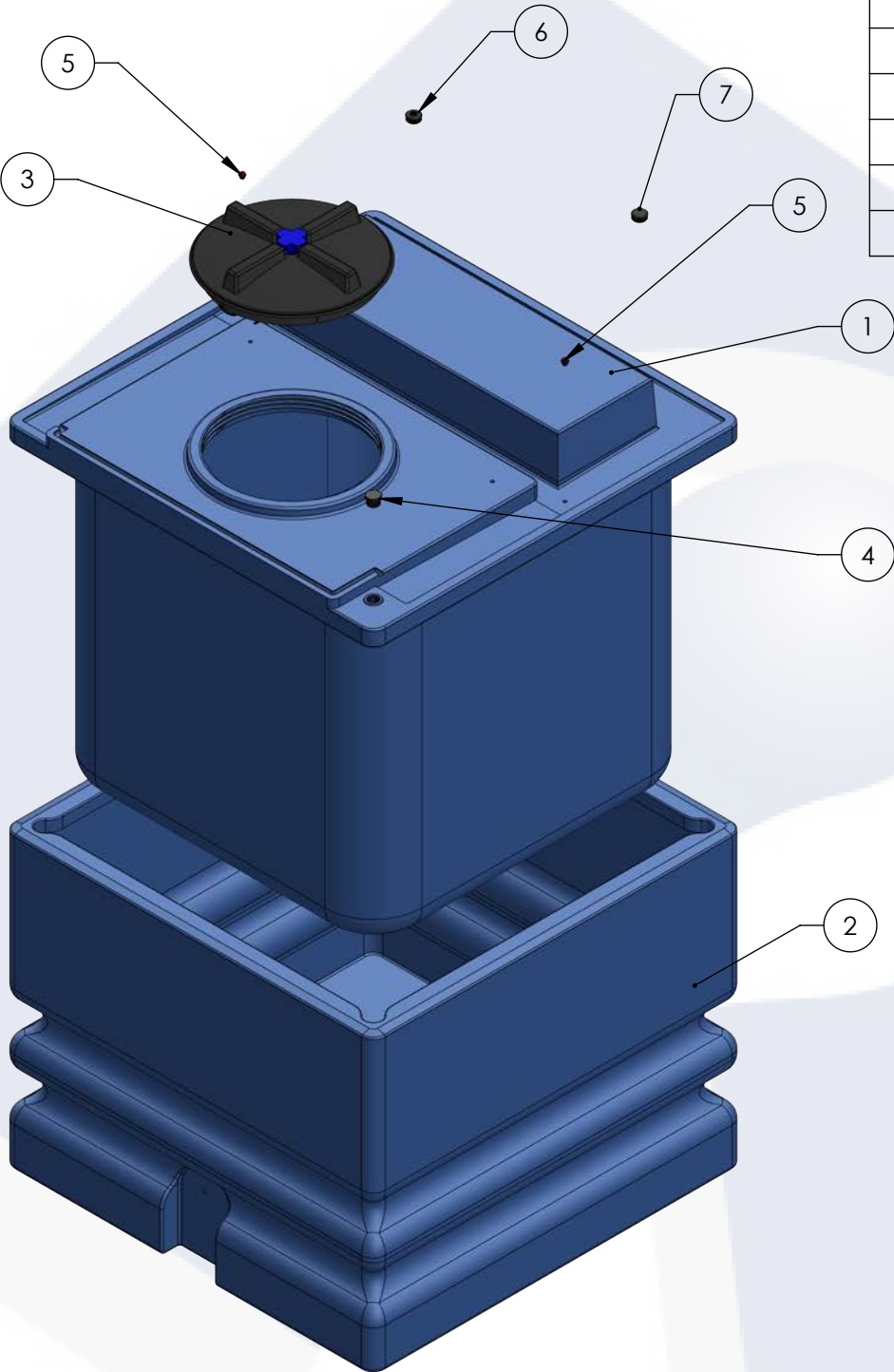
ISOMETRIC VIEW (EXPLODED)
