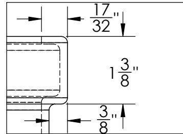
DETAIL B SCALE 1 : 2
