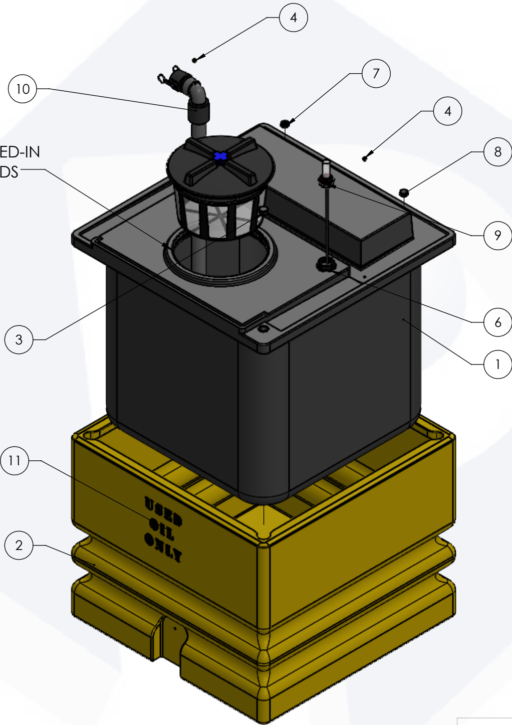
ISOMETRIC VIEW EXPLODED
