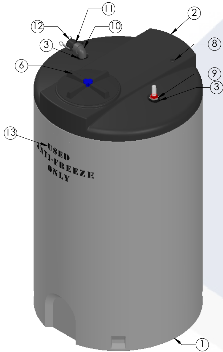
ISOMETRIC VIEW ASSEMBLED
