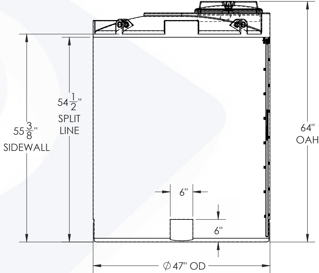
FRONT VIEW
