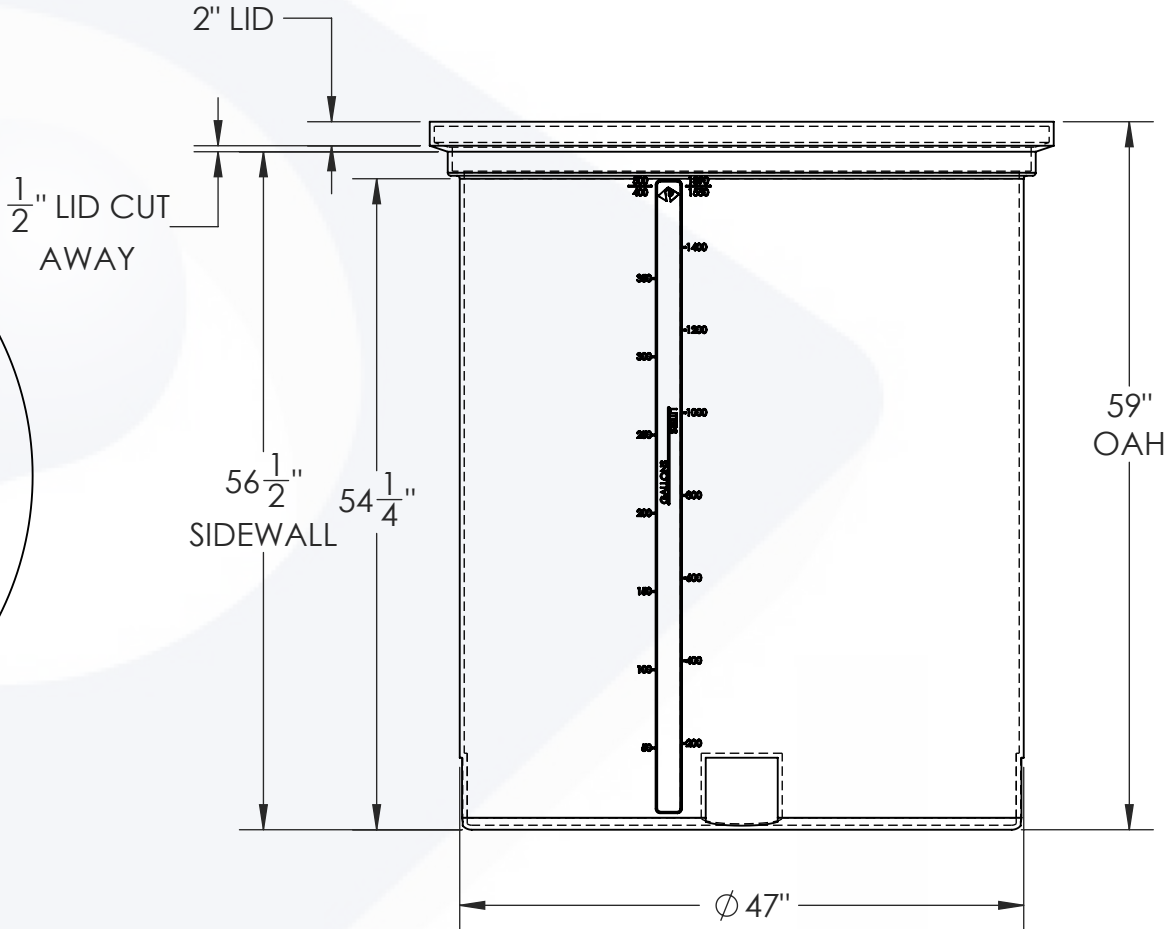
FRONT VIEW
