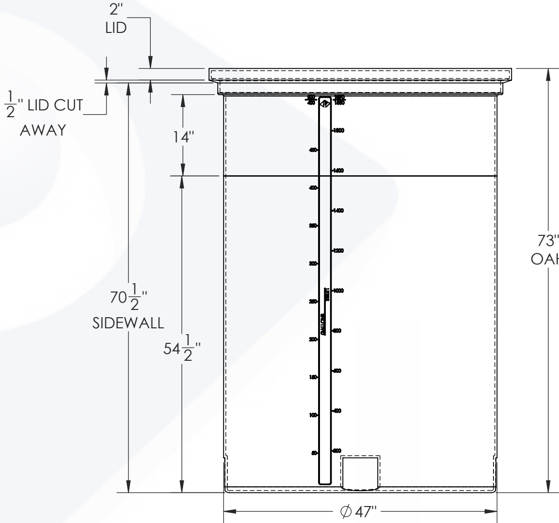
FRONT VIEW
