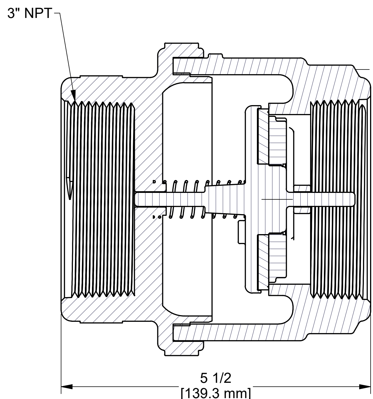
SECTION B-B SCALE 1 : 1
