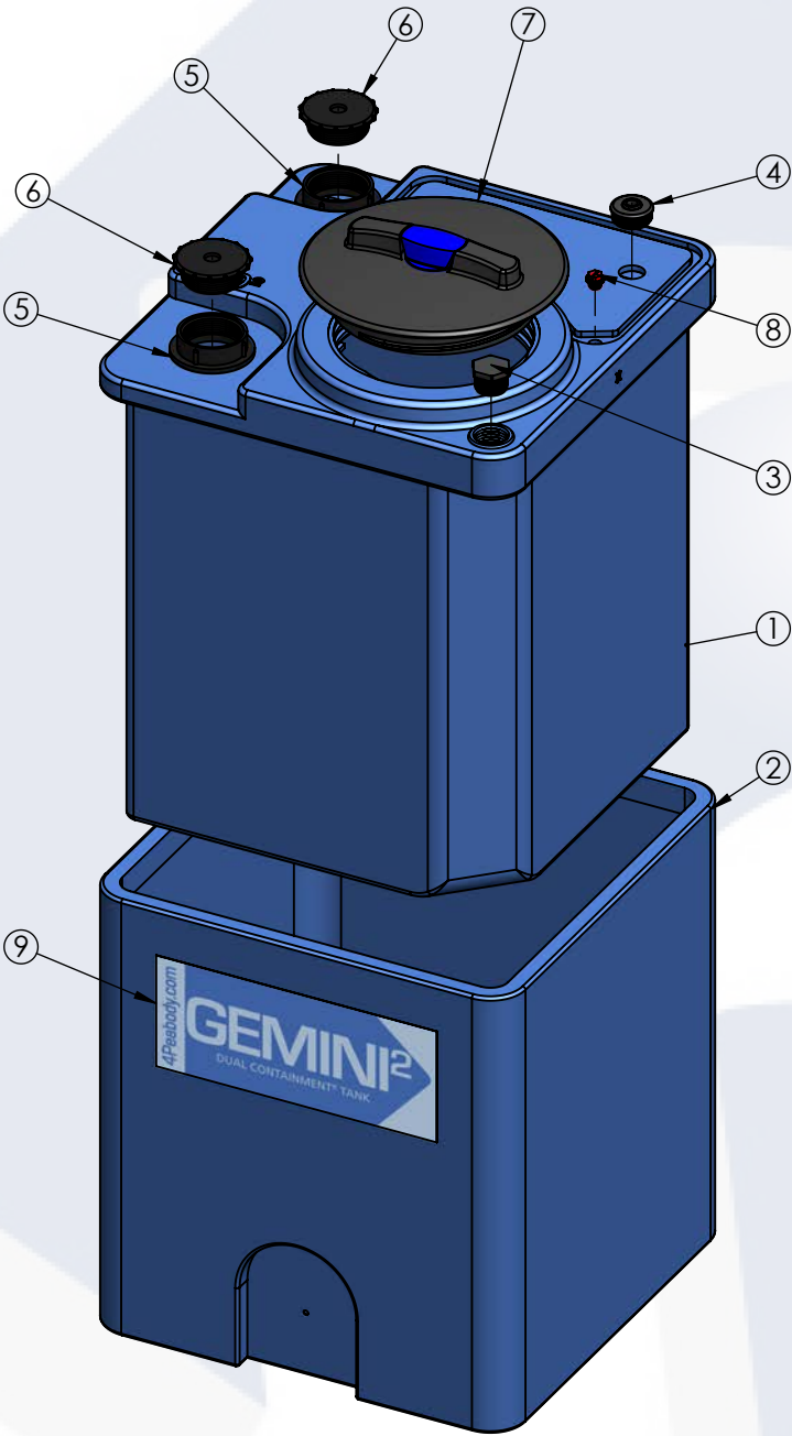
ISOMETRIC VIEW (EXPLODED)
