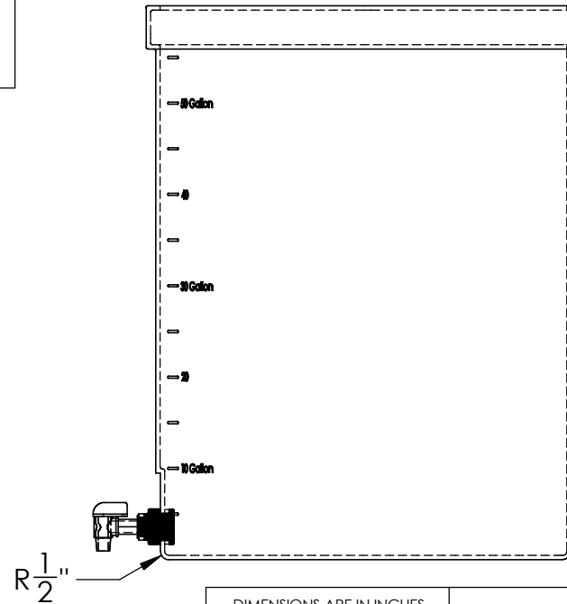
DETAIL A
