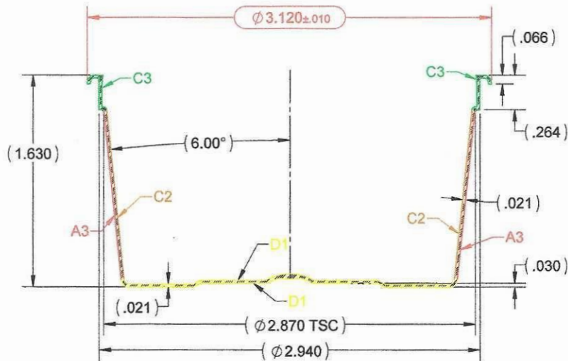
SECTION A-A SCALE 1.5: 1
