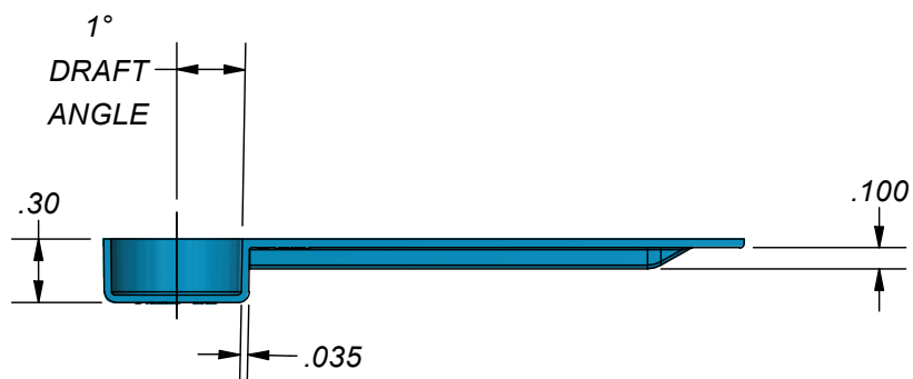
SECTION VIEW
