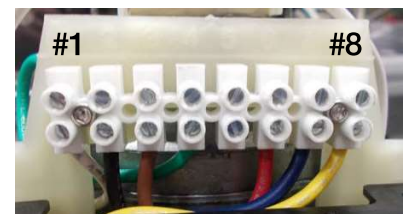
Terminal strips facilitate ease of field wiring and testing.
